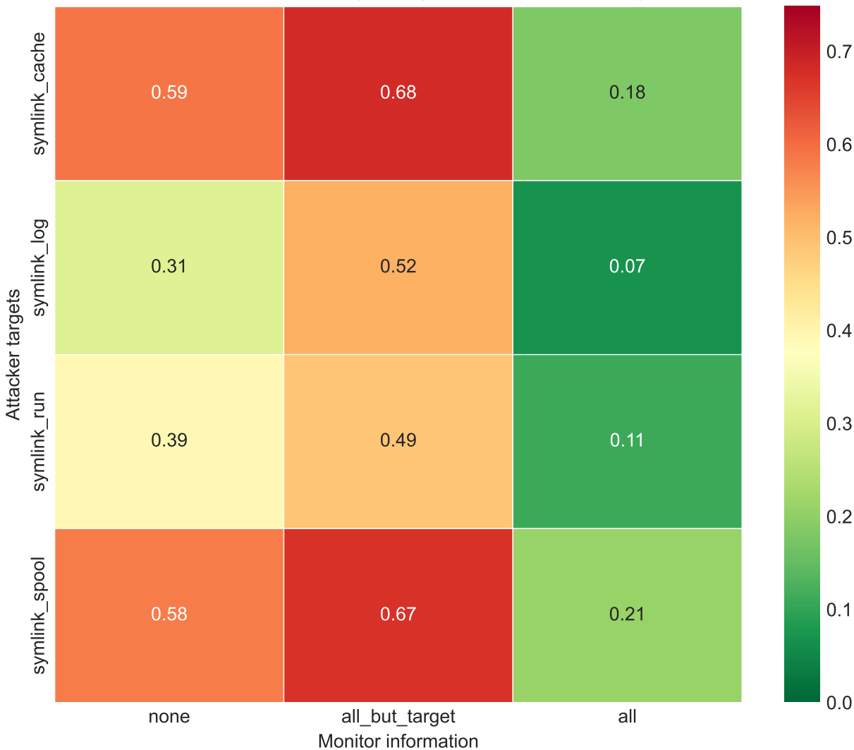
Attack success rate (averaged across thresholds)
